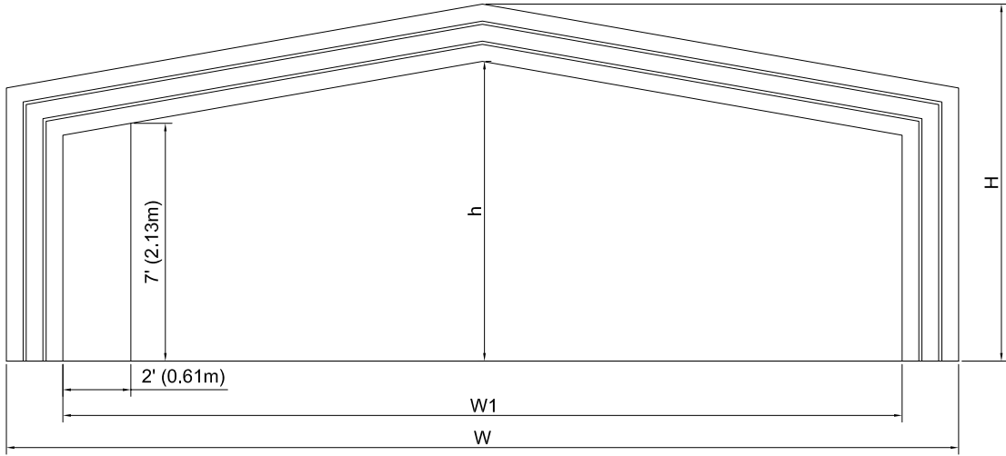
Section View
