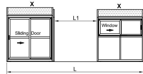
Side Elevation Opened
