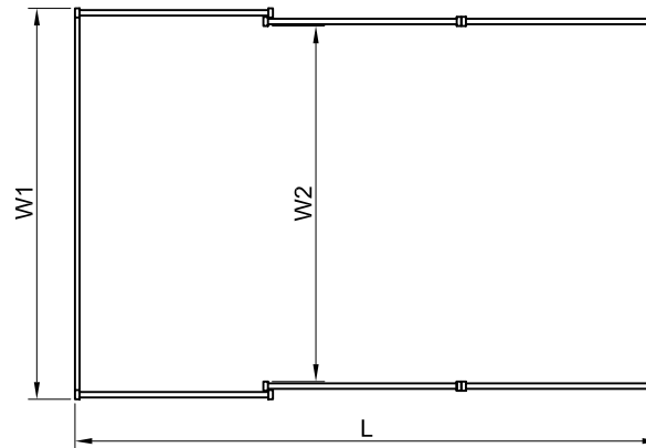
Plan View Section Closed
