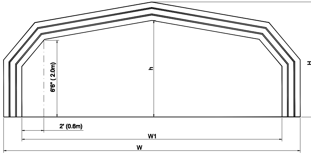
Section View
