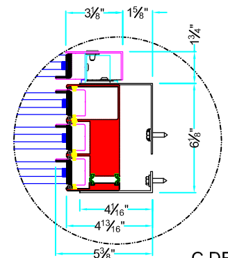
C DETAIL
