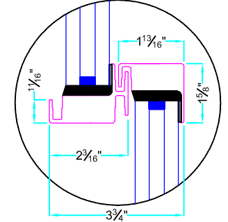
B DETAIL
